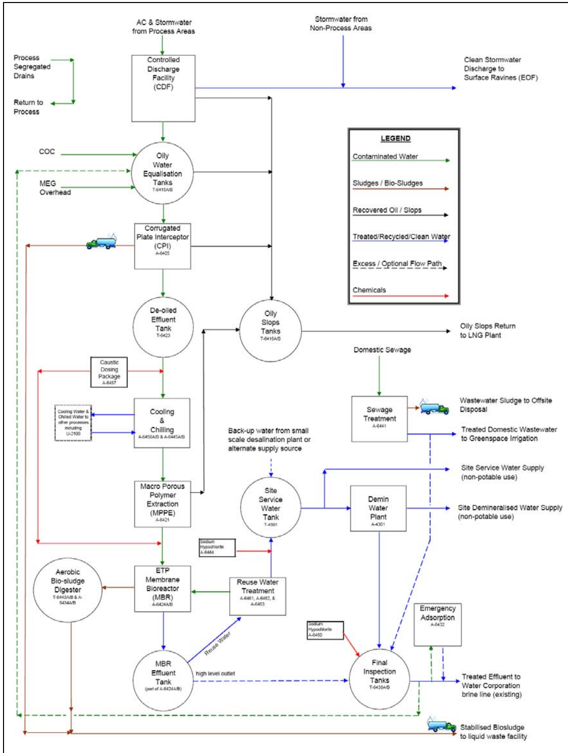
Figure 3-1 Water System Overview
